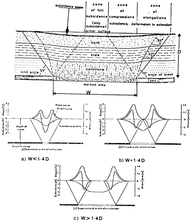
Fig. 1 Component of ground movement at the surface due to total extraction
