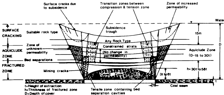
Fig.3. Generalized Depiction of Strata Behaviour with Total Extraction Mining (after Singh and Kendorski, and modified by authors)
