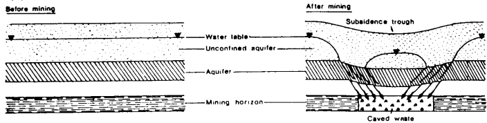
Infiltration of Groundwater Resulting from Mining Subsidence (schematic cross section)
