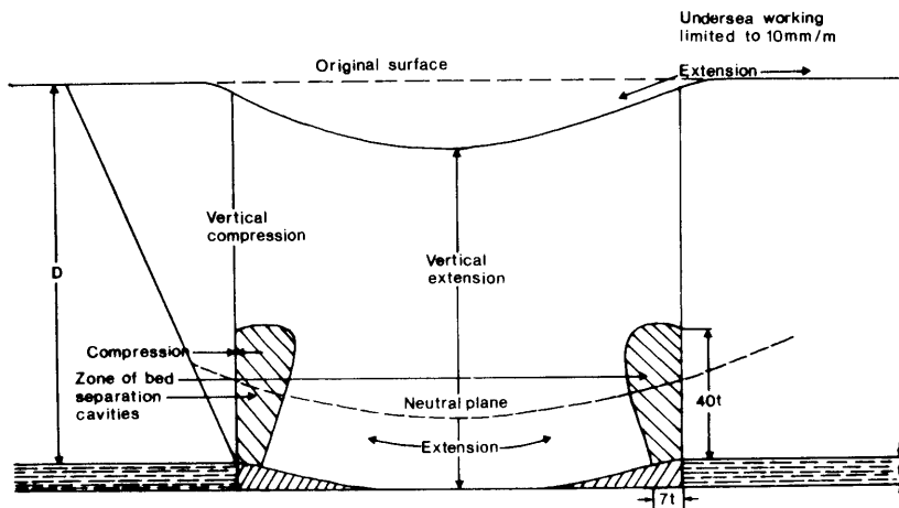
Fig. 2 Schematic Depiction of Stress Zones in Underground Mining
