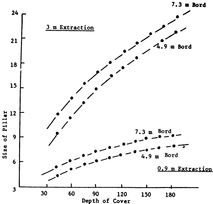
Fig. 12 Design of room and pillar working for undersea working
