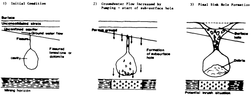
Fig. 5 Formation of Sinkholes in Limestones and Dolomites
