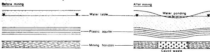
Outcropping of the Groundwater in a Subsidence Trough (schematic cross section)
