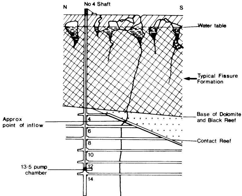
Fig. 7 Section Showing Solution Cavities and Fissure Formation at West Driefontein Mine, S. Africa (after Cousens and Garrett 1969) [8]
