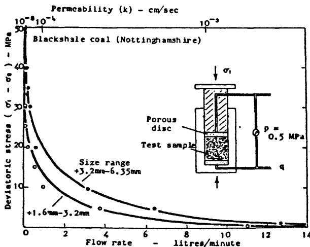
Fig 8 Effect of Stress on Flow Rate Through Broken Coal (after Whittaker and Singh 1978)[11]
