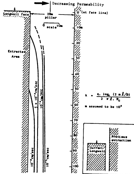
Fig. 9 Rib Pillar Permeability Values from Borehole Tests (after Whittaker and Singh 1978)[11]
