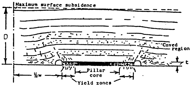
Fig 10 Generalised Representation of Main Fracture Zones Associated with Longwall Mining Rib Pillar (after Whittaker and Singh 1978) [11]
