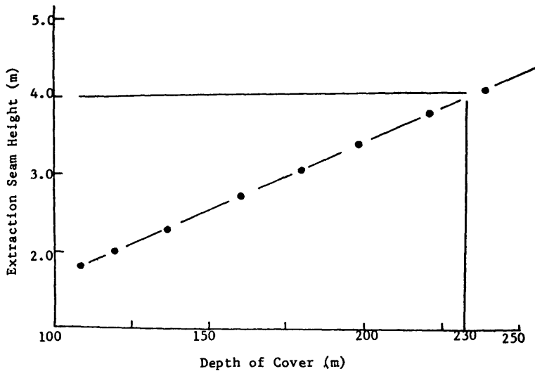
Fig. 11 Working under sea or major aquifer Minimum Depth of cover vs extracted seam ht (Total Extraction Layout)
